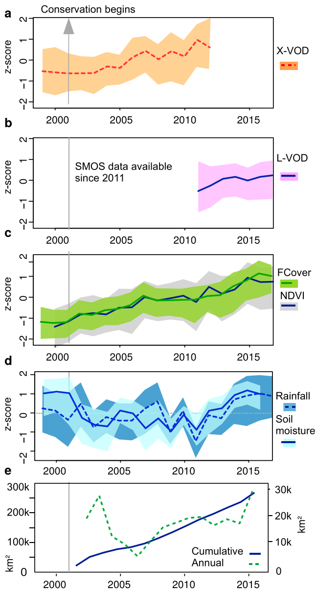
Figure 3. Vegetation and hydrological dynamics 1999–2017 in China karst (Figure 1b). (a) High frequency X-VOD (1999–2012) and (b) low frequency L-VOD (2011–2017). (c) GEOV2 growing season FCover (1999–2017) and MODIS growing season NDVI (2000–2017) together with their 95% confidence intervals (shaded areas). (d) CHIRPS annual rainfall (1999–2017) and CCI soil moisture (1999–2016) with 95% confidence intervals. Annual values are anomalies calculated by the z-score. (e) Annual (right y axis) and cumulative (left y axis) extent of forestry and conservation areas in the eight provinces (2002–2015).
