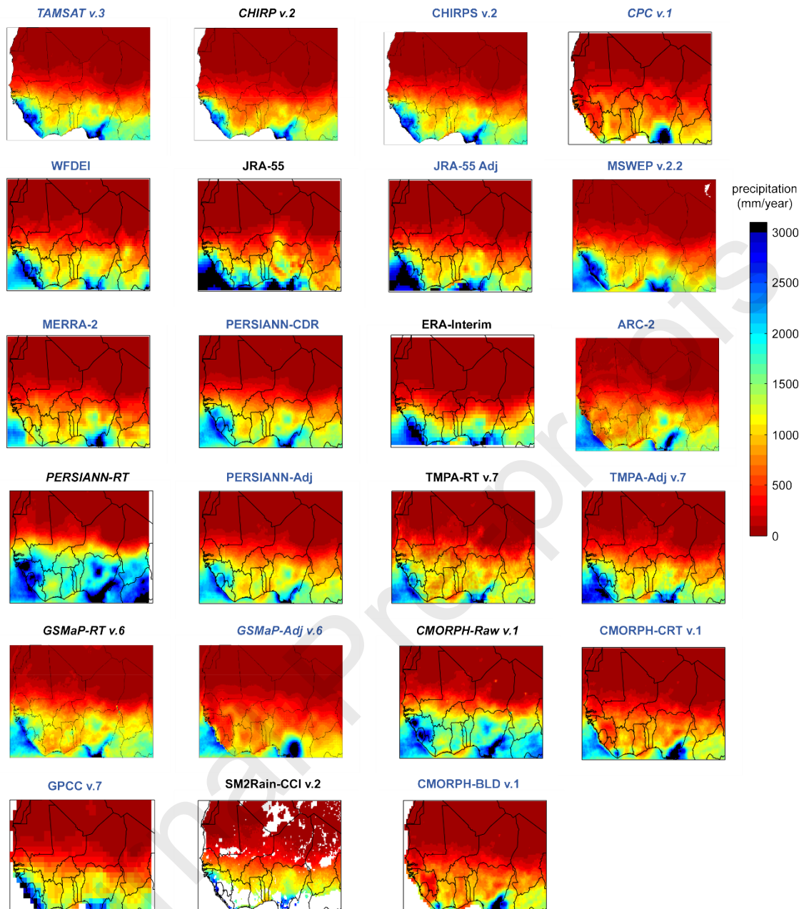
Figure 2. Mean annual precipitation for 2000–2003 retrieved from all P-datasets at their original grid sizes. For each P-dataset, only the grid-cells with more than 80% of available daily data were retained. Blue and black colours are used to highlight P-datasets using and not using gauge-based information, respectively, and italic font is used for P-datasets available in NRT latency of one–three days.
