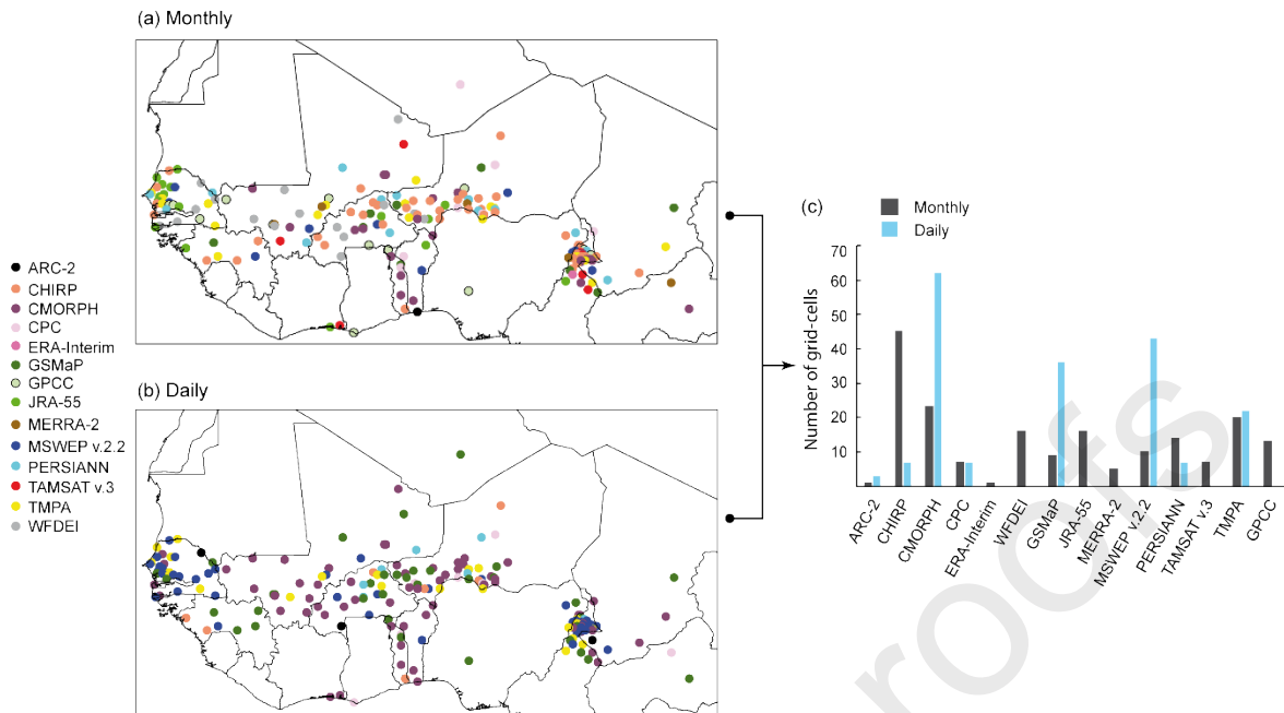
Figure 15. Most efficient P-datasets at the grid-cell level. For simplification, the P-datasets were aggregated in main groups: GSMaP = GSMaP-RT + Adj v.6 ; TMPA = TMPA-RT + TMPA-Adj ; JRA-55 = JRA-55 + JRA-55 Adj ; PERSIANN = PERSIANN-RT + PERSIANN-Adj + PERSIANN-CDR .
