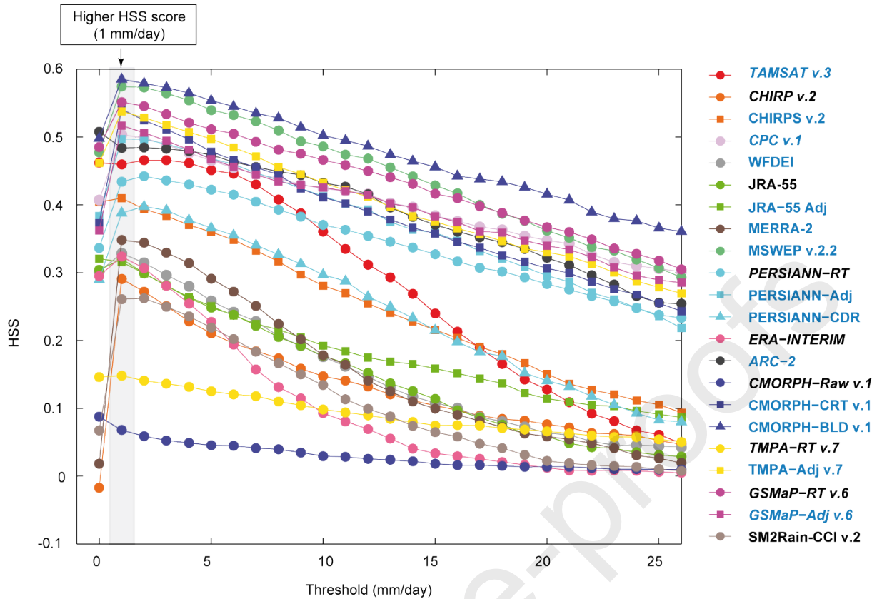
Figure 9. P-dataset ability in reproducing daily precipitation events of different intensities expressed in the form of HSS. Blue and black colours are used to highlight P-datasets using or not using gauge-based information, respectively, and italic font is used for P-dataset available in NRT latency of one to three days.
