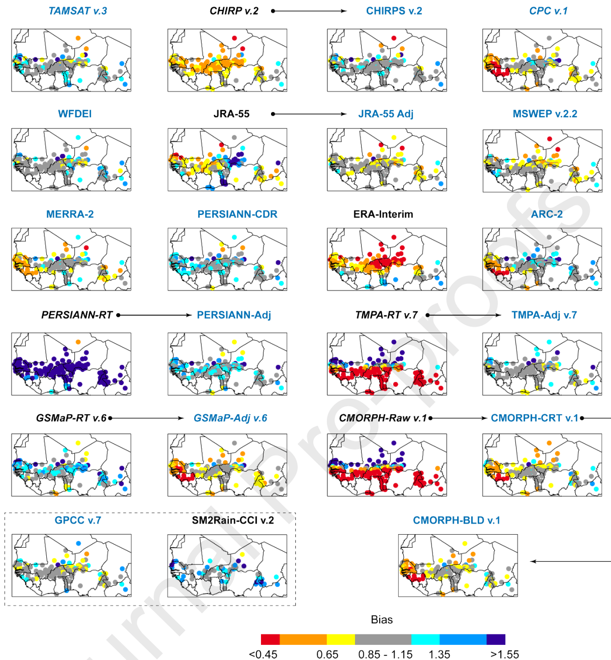
Figure 6. P-dataset reliability at the grid-cell scale expressed in the form of bias considering all months for in 2000–2003. Arrows are used to highlight the potential benefit of using gauge-based information. Blue and black colours are used to highlight P-datasets using or not using gauge-based information, respectively, and italic font is used for P-datasets available in NRT latency of one to three days.
