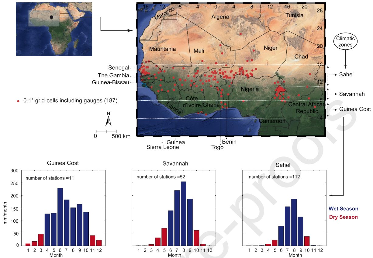
Figure 1. Study area with the considered 0.1^\circ grid-cell locations and the mean monthly precipitation amount given for the three climatic regions based on gauge records of 2000–2003.
