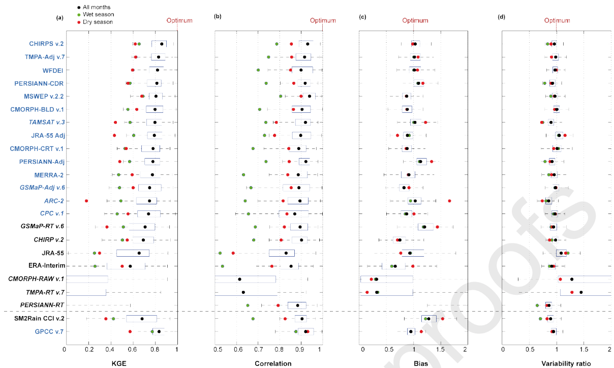
Figure 3. P-dataset reliability at the regional. The right and left edges of the boxes represent the 25th and 75th percentile values, respectively. The P-datasets are sorted from the most (top) to the least (bottom) efficient in term of KGE. SM2Rain-CCI v.2 and GPCC v.7 are at the bottom because their analyses are based on a different number of 0.1^\circ grid-cells, at 79 and 183, respectively. Blue and black colours are used to highlight P-datasets using or not using gauge-based information, respectively, and italic font is used for P-datasets available in NRT latency of one to three days. The graphics were inspired by Beck et al. (2019).
