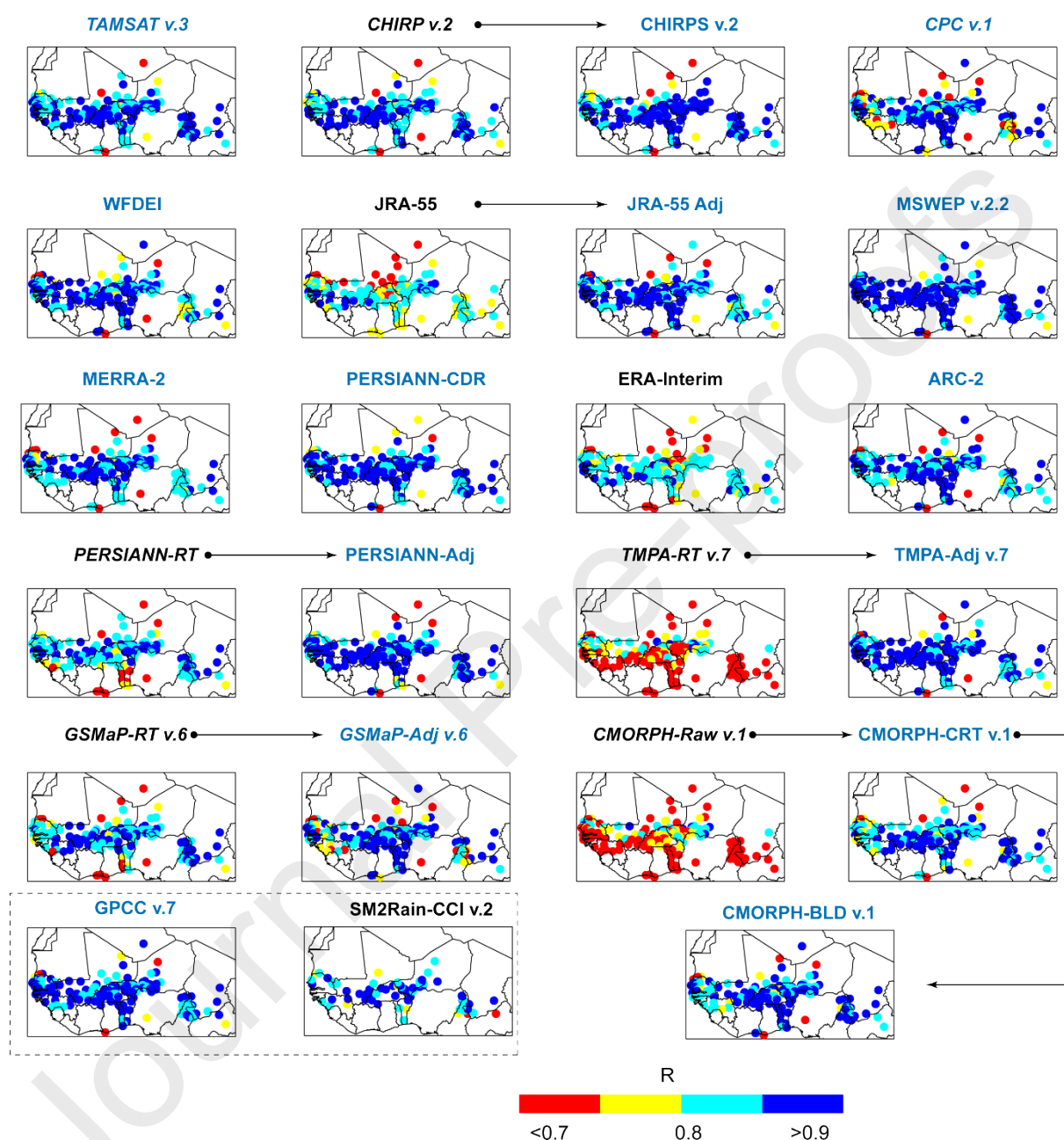
Figure 5. P -dataset reliability at the grid-cell scale expressed in the form of correlation considering all months in 2000–2003. Arrows are used to highlight the potential benefit of using gauge-based information. Blue and black colours are used to highlight P -datasets using or not using gauge-based information, respectively, and italic font is used for P -datasets available in NRT latency of one to three days.
