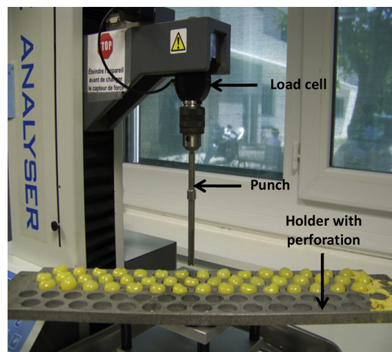
Fig. 1. Sweet cherry disposition and orientation for firmness measurements.
