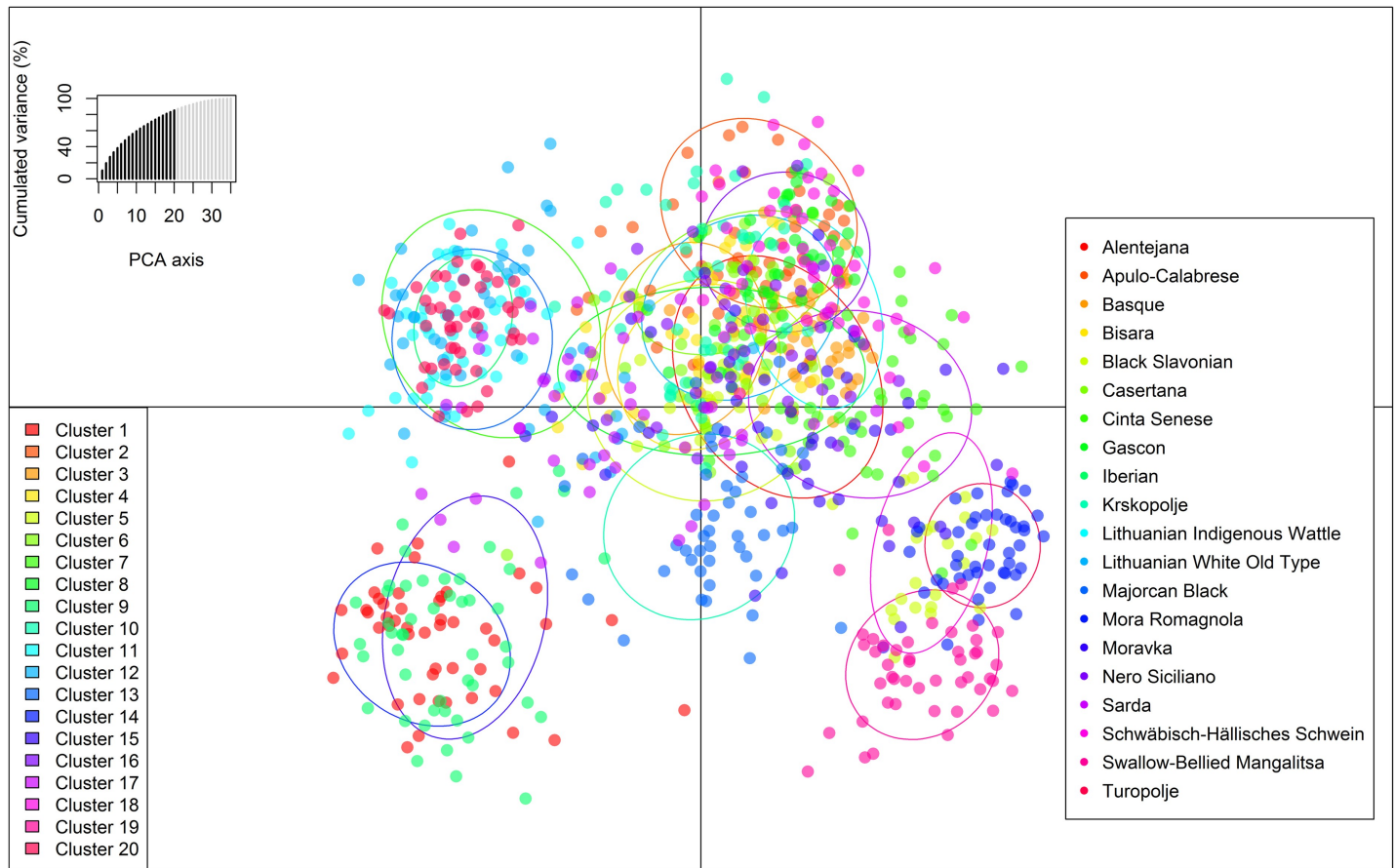
Fig 3. Scatterplot of resulting genetic clusters after Discriminant Analysis of Principal Components for the 20 local European pig breeds.
