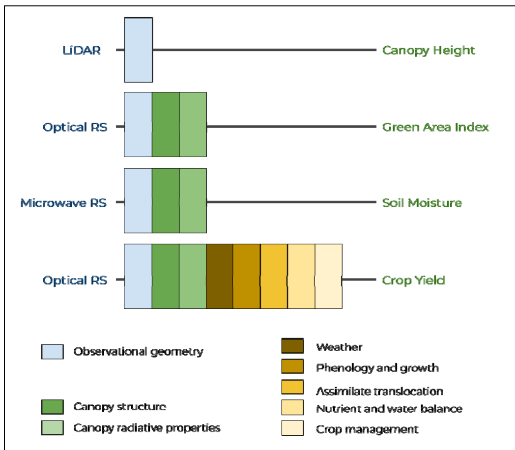
Figure 2. Schematic representation of the level of complexity of the links between remote sensing observations (on the left) and selected agronomic traits of interest (on the right). In the context of this paper, crop height and green area index are considered as primary variables (directly involved in the radiative process) while crop yield is a secondary variable (indirectly accessible from remotely sensed observations). The boxes represent driving factors of different nature that influence this relationship. Optical remote sensing refers to remote sensing over the solar and thermal infrared spectral domains.
