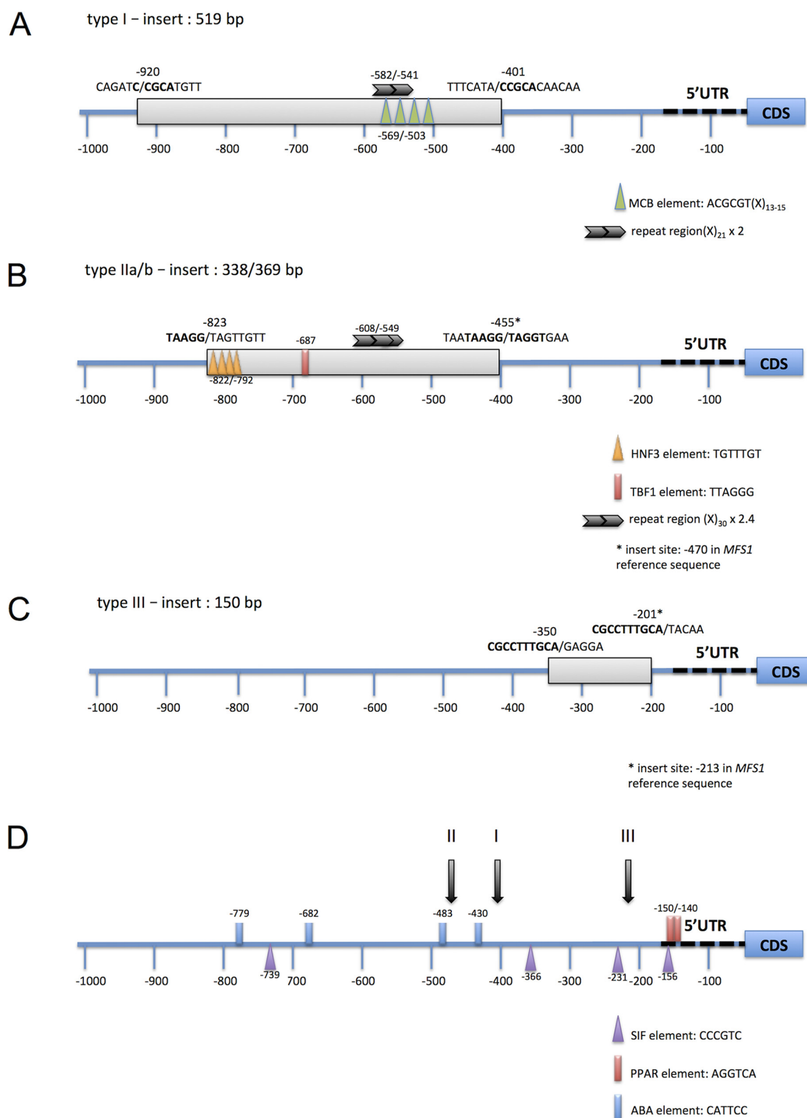
FIG 7 Molecular structure of MFS1 promoter genotypes. The figures indicate the location, length, and insert sites of MFS1 promoter inserts. Repeats between both insertion sites are indicated by boldface letters. Consensus sequences of potential regulatory elements identified by TRANSFAC searches (44) are indicated by the colored triangles and boxes. Repeats of longer sequences, found using mreps (45), are indicated by the black arrows. The MCB element (Mlul cell cycle box) regulates the expression of genes involved in G 1 -phase transition (46). HNF3 is a Rattus norvegicus motif (87, 88). The hexamer TTAGGG corresponds to the S. cerevisiae TBF1 element (89).
