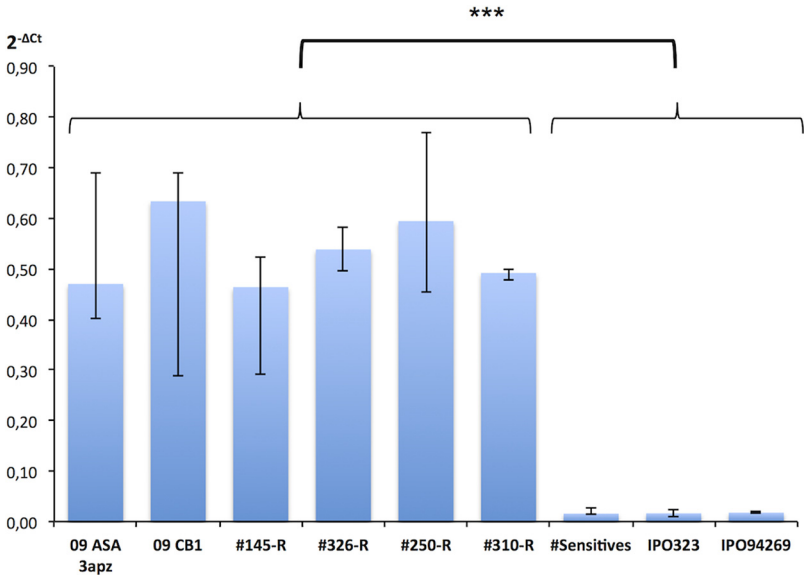
FIG 3 MFS1 expression in parental and progeny strains. MFS1 expression was measured by qRT-PCR relative to three reference genes ( β-tubulin , eF1a , and actin ). Median values ( n = 4 to 12) and interquartile range are indicated in the plot. Progeny strains with an “R” suffix are of the MDR phenotype. The value plotted as “#Sensitives” corresponds to expression data from six independent sensitive strains ( n = 12). ***, significant difference of the MFS1 expression levels between MDR and sensitive strains according to Kruskal and Wallis’ nonparametric statistical test with a risk threshold at 0.1%.
