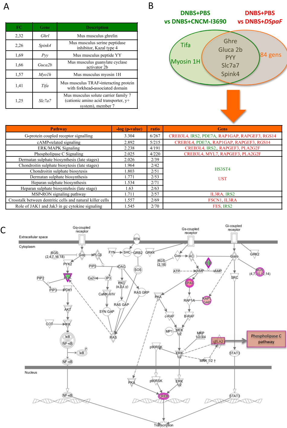
Figure 5. Colonic transcriptome analysis of mice treated with probiotics. Genes modulated by the CNCM I-3690 WT versus DNBS-PBS (A) Genes modulated by the CNCM I-3690 WT versus by the DspaF mutant and the major pathways modulated by DspaF mutant as identified via IPA (B). Representation of G-protein-coupled receptor signaling (including cAMP-related signaling), ERK/MAPK signaling, and phospholipase C signaling (identified and modified via IPA) (C). Genes upregulated and downregulated by the DspaF mutant are in red and green, respectively. Abbreviations: CREB3L4—cAMP responsive element-binding protein 3 like 4; IRS-2—insulin receptor substrate-2; PDE7A—phosphodiesterase 7A; RAP1GAP—RAP1 GTPase-activating protein; RAPGEF3—Rap guanine nucleotide exchange factor 3; RGS14—regulator of G-protein signaling 14; PLA2G2F—phospholipase A2 group IIF; MYL7—myosin light chain 7; HS3ST4—heparan sulfate glucosamine 3-O- sulfotransferase 4; UST—uronyl 2-sulfotransferase; IL3RA—interleukin-3 receptor; FSCN1—fascin actin-bundling protein 1; and FES—fes proto-oncogene.
