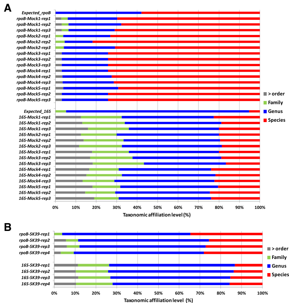
Fig. 1 Impact of the metabarcode markers on OTU taxonomic affiliations. Histogram showing the percentage of OTU affiliations at different taxonomic ranks (x-axis) for rpoB and 16S Illumina-amplicon sequencing for (a) the 15 mock community samples (five mock communities and 3 replicates per mock community) (b) the microbiota of the nematode Steinernema glaseri SK39 (four replicates). Gray, green, blue and red histogram bars correspond to the taxonomic ranks of order (and higher levels), family, genus and species, respectively. The total number of OTUs observed after sequence analysis via the FROGS pipeline was included in the analysis. The Expected_rpoB and Expected_16S lanes correspond to the taxonomic affiliations determined by Sanger sequencing of each of the taxa making up the mock communities
