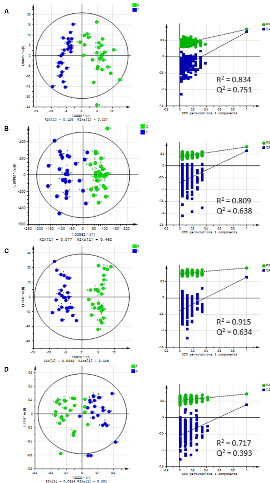
FIGURE 3 | Orthogonal projections to latent structures-discriminant analysis (OPLS-DA) and validation permutation tests of rumen fluid and urine samples from control (C, n = 28 rumen fluid, n = 27 urine) and treated (T, n = 27 ) lambs at 20 weeks of age. (A) Rumen fluid analyzed by LC-MS (284 variables). (B) Rumen fluid analyzed by NMR after variable selection (582 of 641 variables). (C) Urine analyzed by LC-MS (848 variables). (D) Urine analyzed by NMR after variable selection (939 of 1030 variables).
