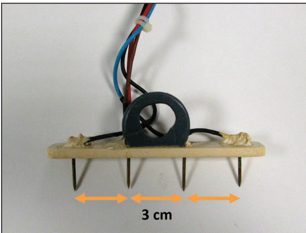
Figure 6 - Electrode quadri-pole built for the pedagogic device with a distance of 3 cm between electrodes (Giot G., 2009).
