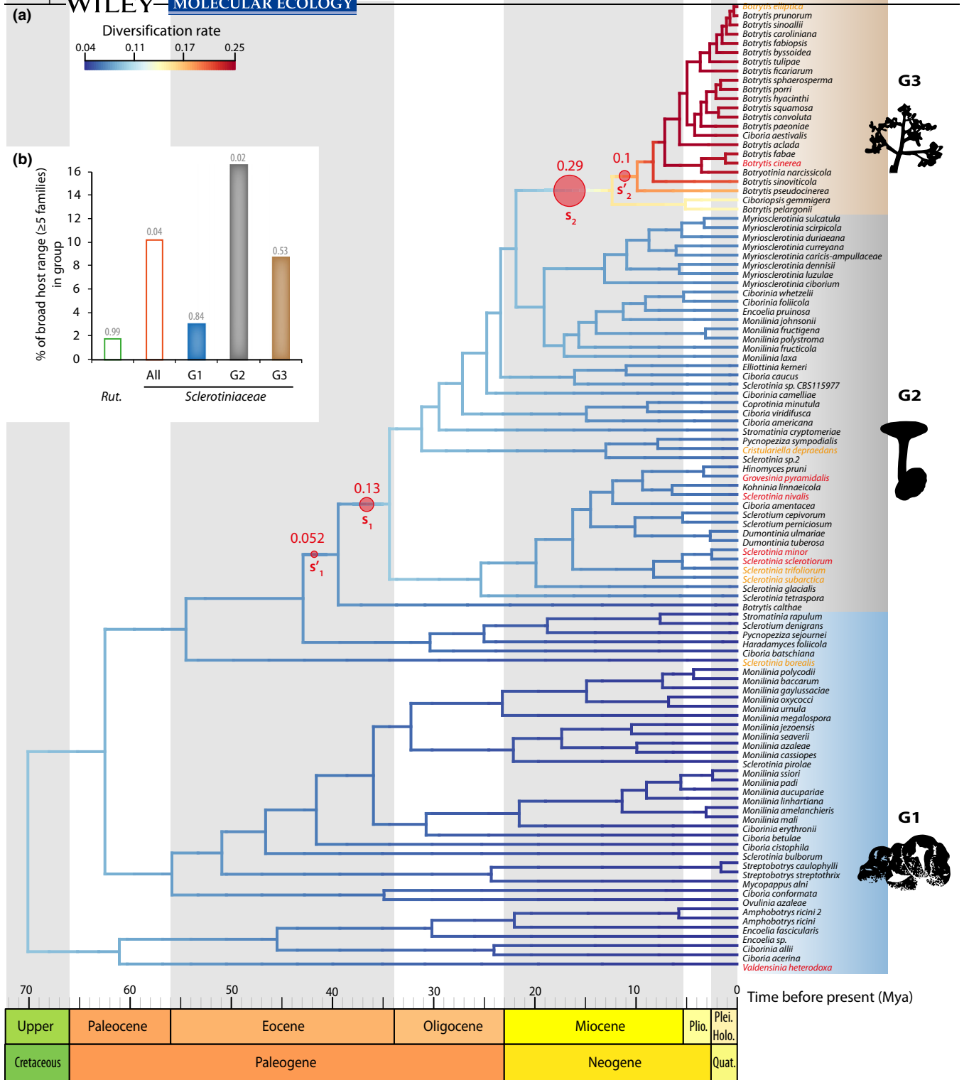
FIGURE 2 Two major diversification rate shifts in the evolution of the Sclerotiniaceae . (a) Dated ITS-based species tree for the Sclerotiniaceae with diversification rate estimates. The divergence times correspond to the mean posterior estimate of their age in millions of years calculated with BEAST. Mean age is shown for selected nodes with bars showing 95% confidence interval of the highest posterior density (HPD). Branches of the tree are colour-coded according to diversification rates determined with BAMM. Major rate shifts identified in BAMM are shown as red circles, noted s_1 , s_1' , s_2 and s_2' and labelled with the posterior distribution in the 95% credible set of macro-evolutionary shift configurations. Species names are shown in black if host range includes less than five plant families, in yellow for five to nine plant families and in red for 10 or more plant families. Diversification rate shifts define three macro-evolutionary regimes noted G1, G2 and G3 and boxed in blue, grey and brown, respectively. (b) Distribution of broad host range (five or more host families) parasites in Rutstroemiaceae , Sclerotiniaceae and under each macro-evolutionary regime of the Sclerotiniaceae . p -Values calculated by random permutations of host ranges along the tree are indicated above bars. Holo., Holocene; Mya, Million years ago; Plei., Pleistocene; Plio., Pliocene; Quat. Quaternary; Rut., Rutstroemiaceae [Colour figure can be viewed at wileyonlinelibrary.com ]
