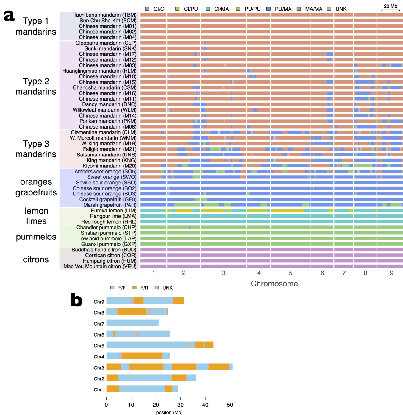
Extended Data Figure 2 | Segmental ancestry and admixture in citrus.
