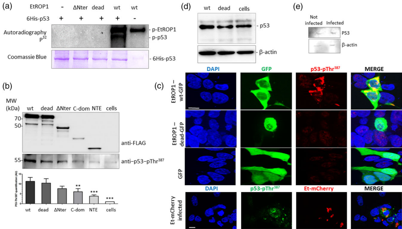
FIGURE 4 EtROP1 phosphorylates p53 on residue Thr 387 . (a) SDS-PAGE autoradiography of a kinase assay (top panel) performed on EtROP1-FLAG recombinant proteins (WT, dead and \Delta\text{Nter} forms) and a 6His-tagged p53 recombinant protein (detected by SDS-PAGE followed by Coomassie blue staining, bottom panel). (b) Western blot analysis showing p53 phosphorylated Thr 387 residue (p53-pThr 387 ) co-purification with EtROP1-FLAG wt, dead, \Delta\text{Nter} , C-dom and NTE forms in a pull-down assay using anti-FLAG affinity-chromatography after constructs transfection in HEK293T cells. EtROP1-FLAG constructs (wt, dead, \Delta\text{Nter} , C-dom and NTE; top panel) and p53-pThr 387 (bottom panel) were detected using an anti-FLAG or an anti-p53-pThr 387 antibody, respectively. Western blot signal were quantified by densitometry and ImageJ. (c) Upper panel: fluorescence microscopy analysis showing GFP (green) and phosphorylated p53 (anti-p53-pThr 387 antibody, red) detection in HEK293T cells transfected with EtROP1-GFP expression plasmids (wt and dead forms) or the control plasmid pcDNA-GFP. Lower panel: phosphorylated p53 (anti-p53-pThr 387 antibody, green) detected in HEK293T cells infected with E. tenella expressing mcherry (red). Bar represents 10 \mu\text{m} . (d) Western blot analysis showing p53 stabilisation in HEK293T cells transfected with EtROP1-GFP expression plasmids (wt and dead forms) or the control plasmid pcDNA-GFP. Two days posttransfection, GFP positive cells (transfected cells) were flow cytometry sorted before immunoblot analysis using an anti-p53 antibody. An anti- \beta -actin antibody was used as an internal standard of immunoblot (IB). (e) Western blot analysis showing p53 stabilisation in epithelial caecal cells infected with E. tenella . Eighty-four hours postinfection, mCherry positive caecal cells (infected cells) were flow cytometry sorted for subsequent total RNA purification. Analysis was run as in 4D legend
