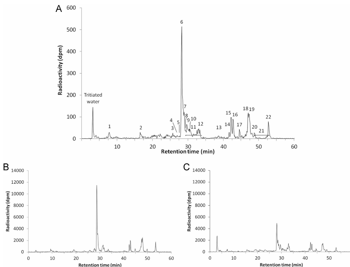
Fig. 5. Radio-HPLC profiles of ^3\text{H} -HNE urinary metabolites after oral administration in rats. A: 0–24 h urine. B: 0–6 h urine. C: 6–24 h urine.
