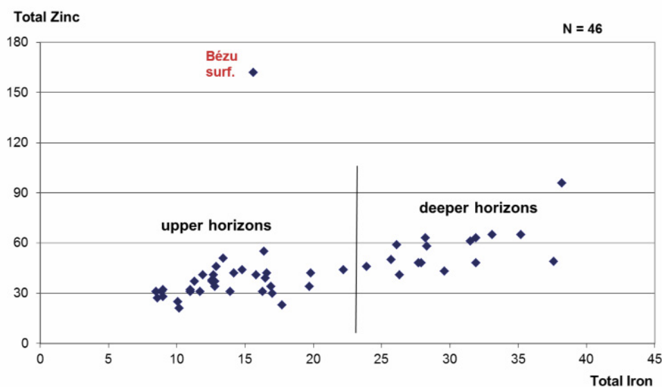
Figure 3. Albeluvisols developed in a loamy aeolian deposit (South-east of the Paris basin). Forty six samples were taken at different depths from forest and cultivated soils. Upper horizons were taken at 0 to 45 cm depth – deeper ones at 50 to 110 cm depth. Strong natural correlation between total concentrations of Zn and Fe was observed. One sample, outside this correlation is the surface Ap horizon of the experimental plot at Bézu-le-Guéry amended with sewage sludge at high rates (Baize and VanOort, 2014)
