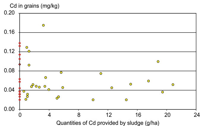
Figure 6. Trials in Burgundy and Franche-Comté (Deléan and Kockmann, 2003). Relationship between cadmium content in wheat grains and Cd quantities provided by sewage sludge application ( R^2 = -0.016 ). Cadmium-input in 15 control plots are nil.
