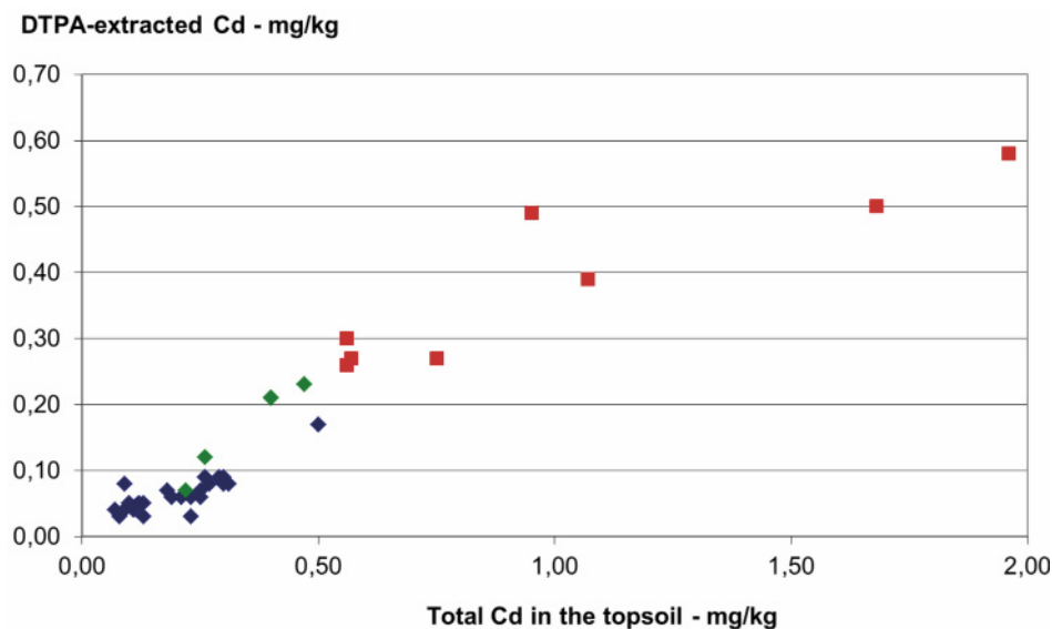
Figure 4. Soils of the Limoges area (36 ploughed horizons). Relationship between cadmium extracted with DTPA and total Cd in topsoil samples. “Large quantities” sites are shown by red squares, “moderate quantities” by green diamonds and “small quantities” and control sites by blue diamonds (Courbe et al., 2002)
