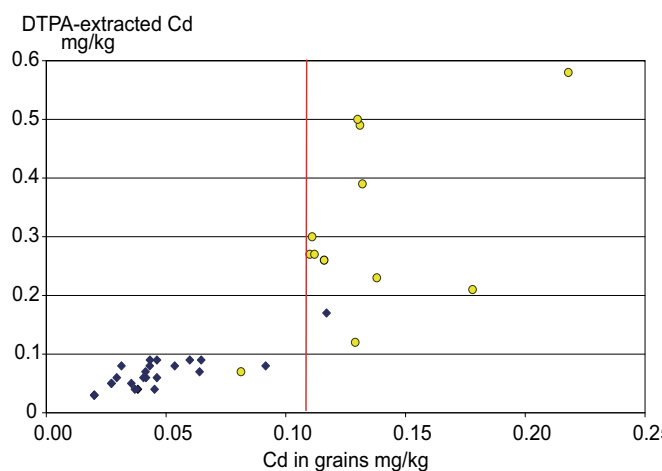
Figure 5. Soils of the Limoges area (36 ploughed horizons). Relationship between cadmium extracted with DTPA from soil samples and cadmium assayed in wheat grains. “Moderate and large quantities” sites are shown by yellow circles; diamonds represent the control sites and the two “small quantities” sites (Courbe et al., 2002). The red line corresponds to the French recommended maximal value
