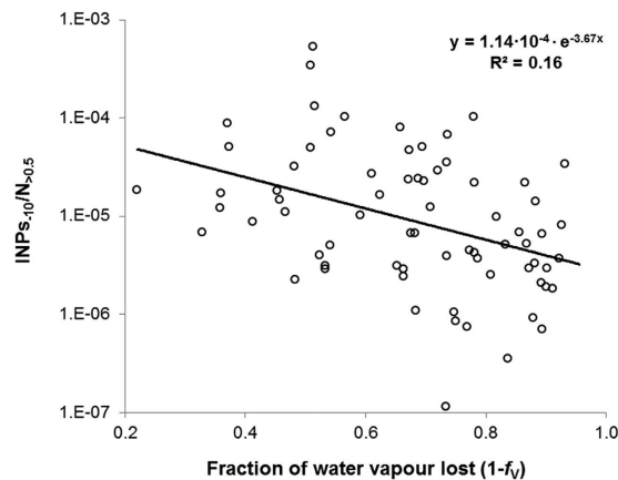
Figure 3. Ratio of INPs -10 to the total number of particles >0.5 μm ( N_{>0.5} , on log scale) as a function of the fraction of water vapour lost from the air mass prior to arrival at the observatory ( n = 71 , Spearman's r = -0.42 , p < 0.001 ).
