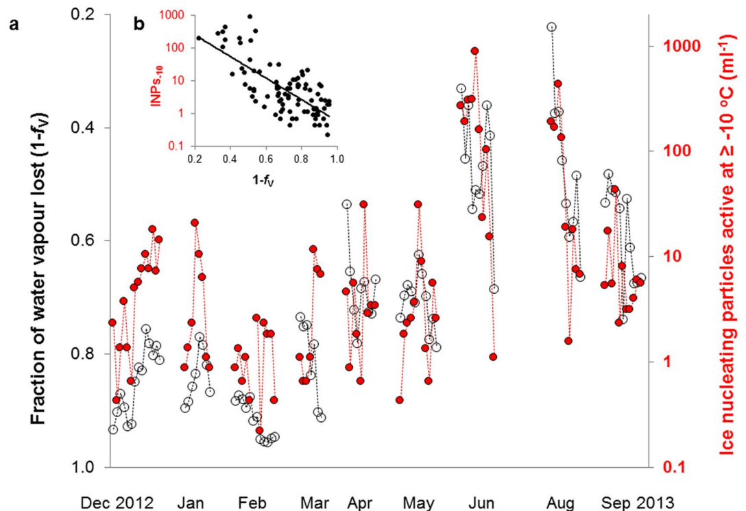
Figure 2. (a) Covariation over time of concentrations of INPs -10 in snow (red, log scale) and the estimated fraction of water vapour lost from an air mass prior to its arrival at the Jungfraujoch observatory (black). Time proceeds from left to right, intervals are not to scale. Each symbol signifies a snow sample with a median sampling duration of 2 hours. Each campaign (symbols connected by dotted lines, one campaign per month) lasted from 3 to 5 subsequent days. A total of 91 samples were collected between December 2012 and September 2013 (exception of July 2013 due to the lack of considerable precipitation events); (b) Relationship between INPs -10 and 1-f_v ; the function of the fitted exponential curve is reported in equation (1).
