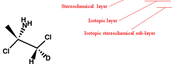
FIGURE 4 | Example of InChIs with no formula layer (1) or with isotopic layer repeated (2). (adapted from InChI Technical Frequently Asked Questions).
