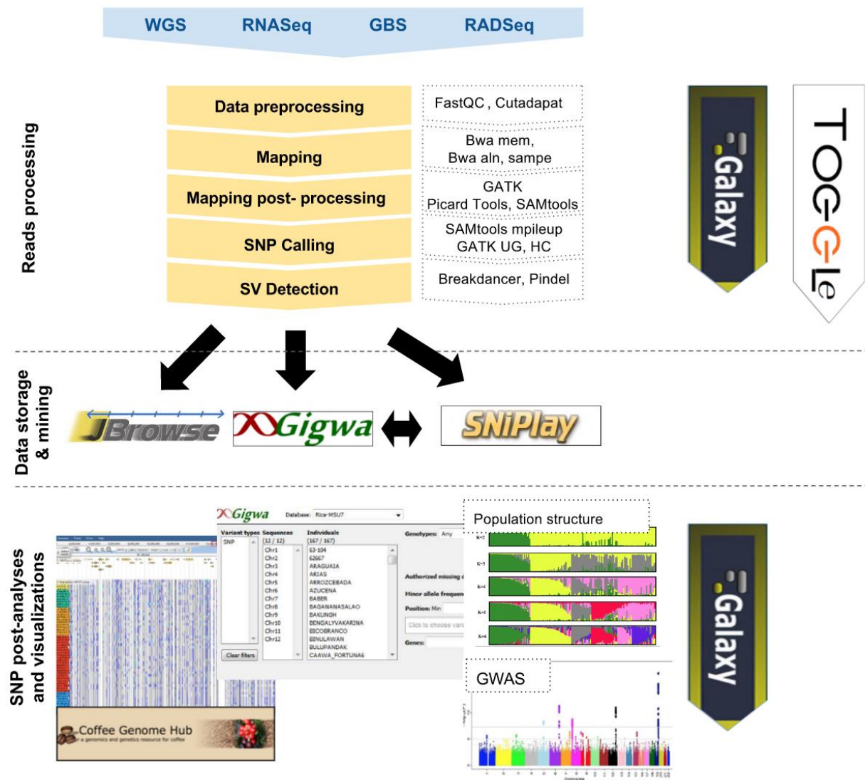
Figure 1. South Green resources and strategy to process, analyze and display Next-Generation Sequencing datasets in the context of genomic variation studies.
