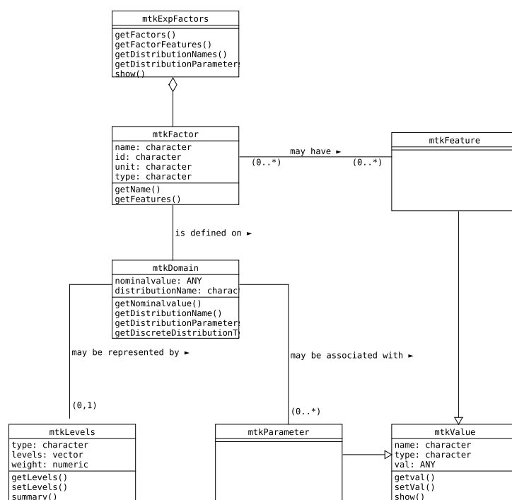
Figure 3: Data model used to manage the factors and their uncertainties. The model is represented using the UML notation (Fowler, 2003), and the referred classes are presented in Table 1.
