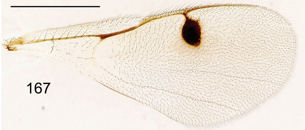
Figures 163–167. Megastigmus somaliensis Hussey. 163 lateral view of female body 164 electroscan of front view of male head 165 electroscan of male antenna 166 electroscan of dorsal view of male thorax 167 male forewing.
