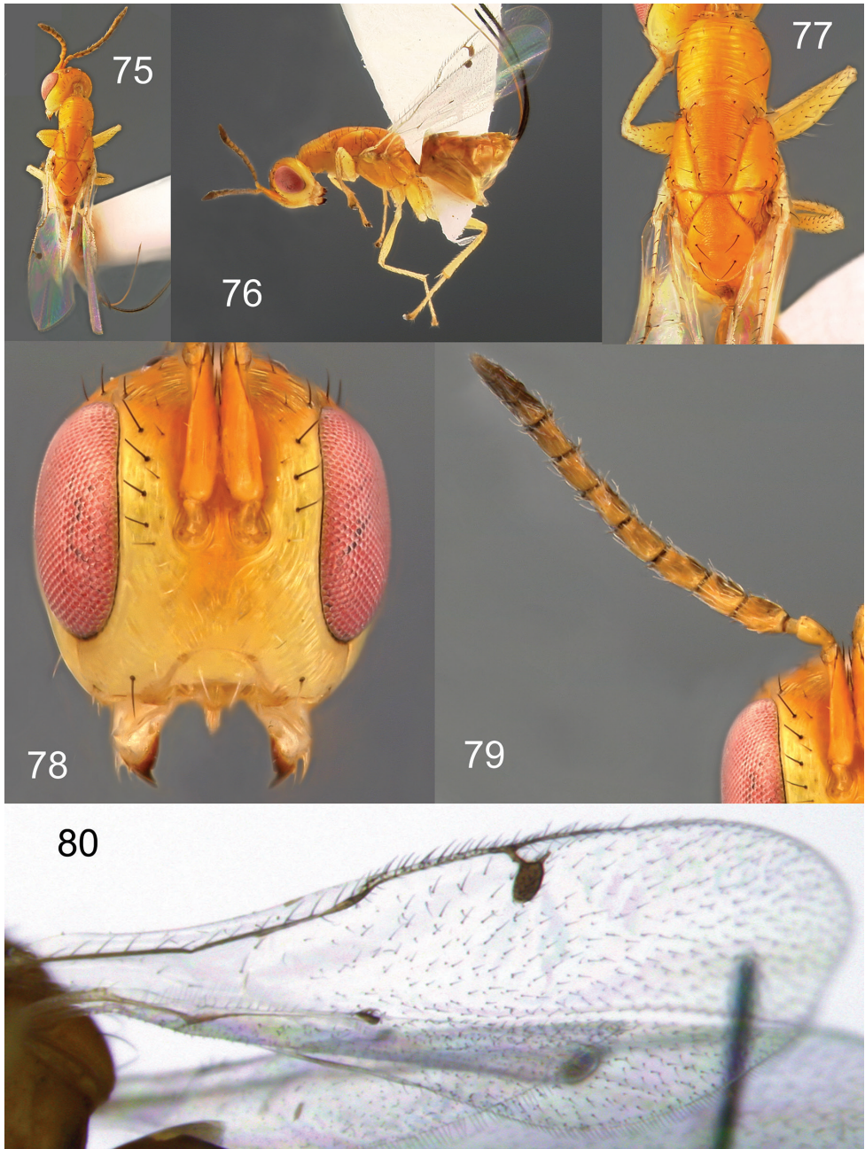
Figures 75–80. Megastigmus laventhami Roques & Copeland, sp. n. female. 75 dorsal view of the body 76 lateral view of body 77 dorsal view of thorax 78 front view of head 79 antenna 80 forewing.
