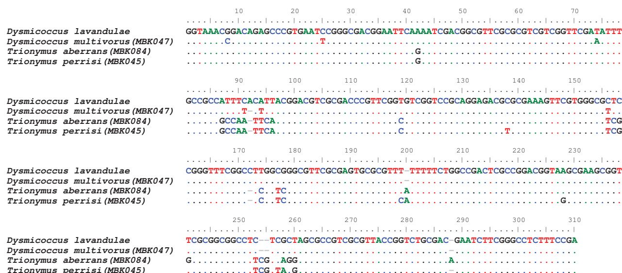
FIGURE 5. Alignment of the 28S DNA sequences obtained for D. lavandulae and already available for other Dysmicoccus and Trionymus species. D. lavandulae is used as reference sequence in the alignment and only the differences to this reference are displayed in the sequences of the other species. The voucher code for the previously available sequences (Kaydan et al. 2015) are given in brackets.
