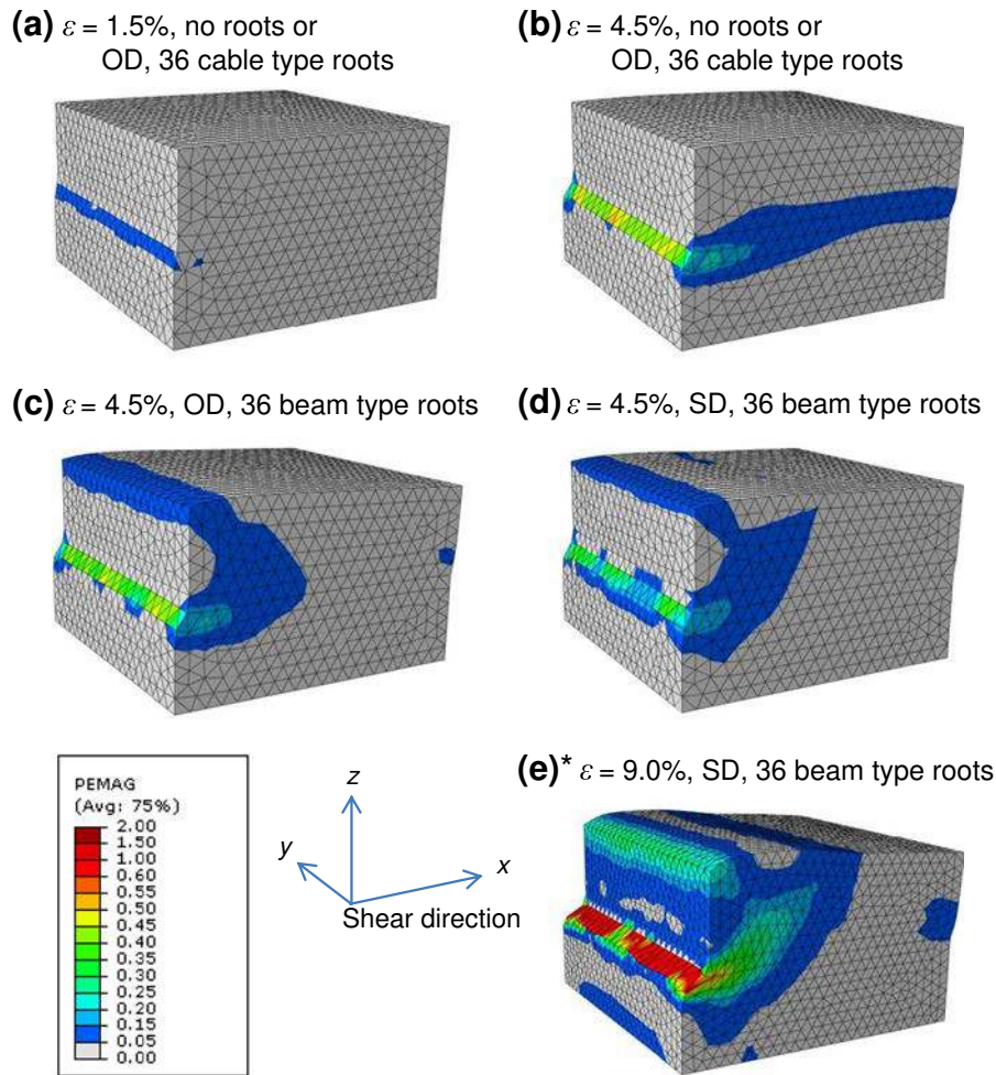
Fig. 8 Visualisation of soil plastic strains for non rooted and rooted soils. PEMAG = plastic strain magnitude; *: a seed density of 0.020 m in mesh was used rather than a density of 0.025 m
