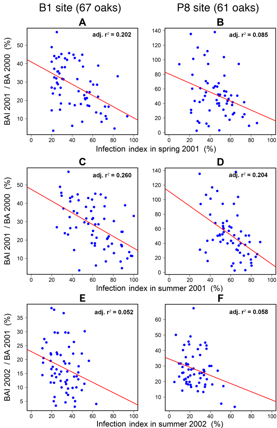
Fig 5. Growth index BAI_n/BA_{n-1} as a function of infection index for two years and two sites.
