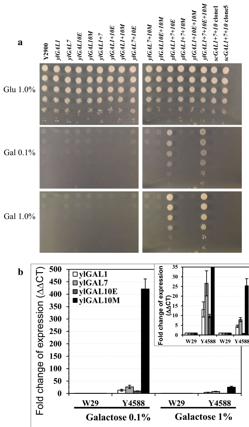
Fig. 6 Functional analysis of Leloir pathway overexpression in Y. lipolytica and fold change in the expression of the yI GAL genes. Growth of different Y. lipolytica transformants overexpressing yI GAL and scGAL genes on plates of YNB medium containing glucose or galactose—incubation at 28 °C, 48 h ( a ). Fold changes in the expression of yI GAL genes in the quadruple mutant, Y4588 (in which all the Leloir genes were overexpressed), relative to Y. lipolytica W29 (the wild-type strain) ( b ); yeast were incubated for 3 h in YNB medium containing 0.1 or 1.0 % galactose. Gene expression levels were normalized based on the expression of the actin gene
