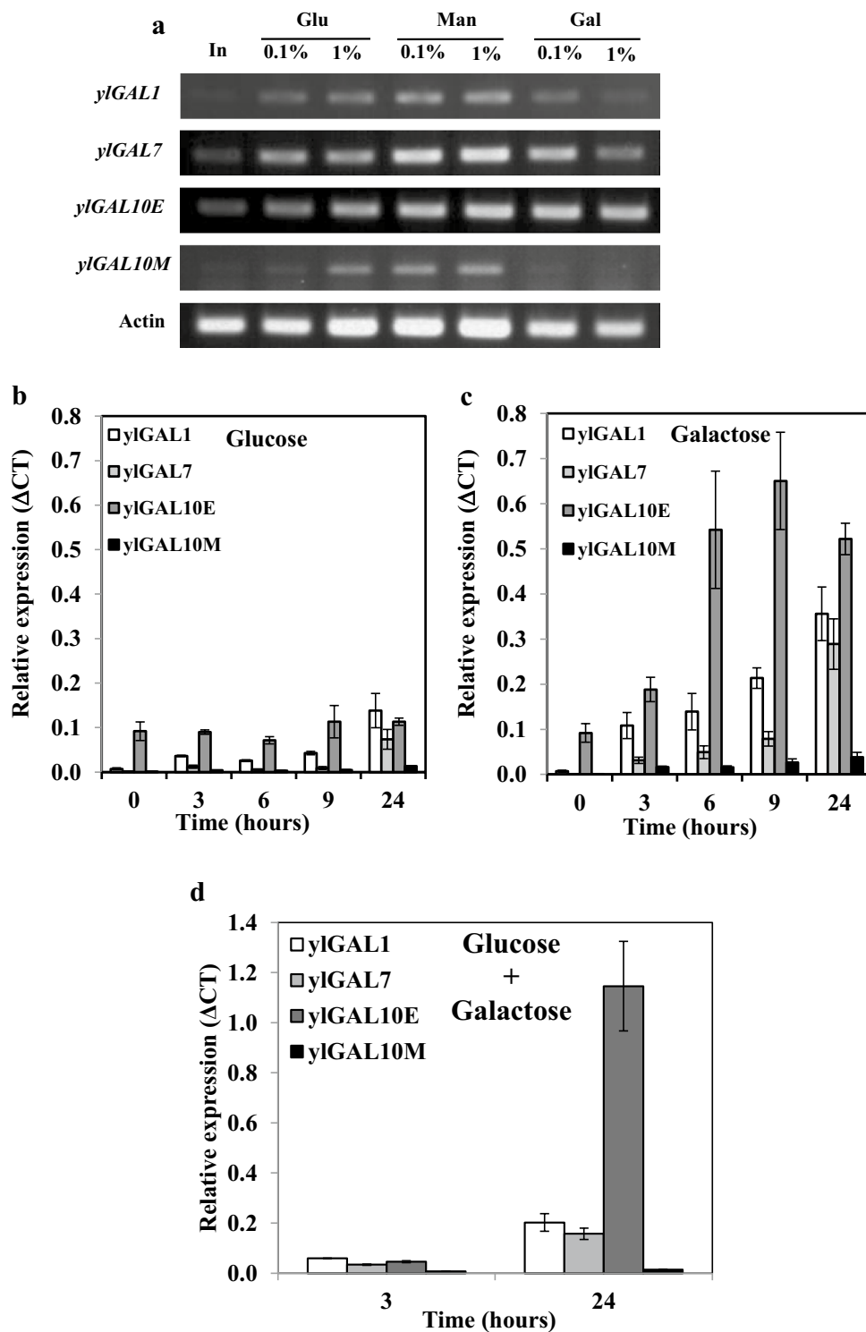
Fig. 2 Expression profiles of yI GAL genes in Y. lipolytica W29. Cells were first growing for 16 h in YNB medium with 1.0 % of glucose and then incubated for 3–24 h in YNB medium containing the indicated sugar at 0.1 or 1.0 %. End-point RT-PCR was performed after 3 h incubation in glucose, mannose, or galactose ( a ). Kinetics of yI GAL genes expression was monitored by quantitative RT-PCR in Y. lipolytica W29 incubated in YNB medium containing 1.0 % glucose ( b ), 1.0 % galactose ( c ), or a mixture of 1.0 % glucose and 1.0 % galactose ( d ). Gene expression levels were normalized based on the expression levels of the actin gene ( \Delta C_T ). In inoculum
