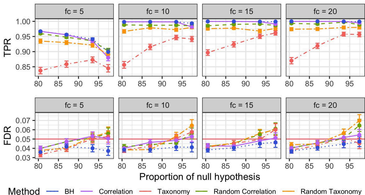
FIGURE 5 | Mean and Squared Error of the Mean (SEM) of the true positive rates TPR (Top) and FDR (Bottom) per different fold changes (facets) for non-parametric simulations. The different FDR control procedures are color-coded. Mean and SEM are computed over 600 replicates.
