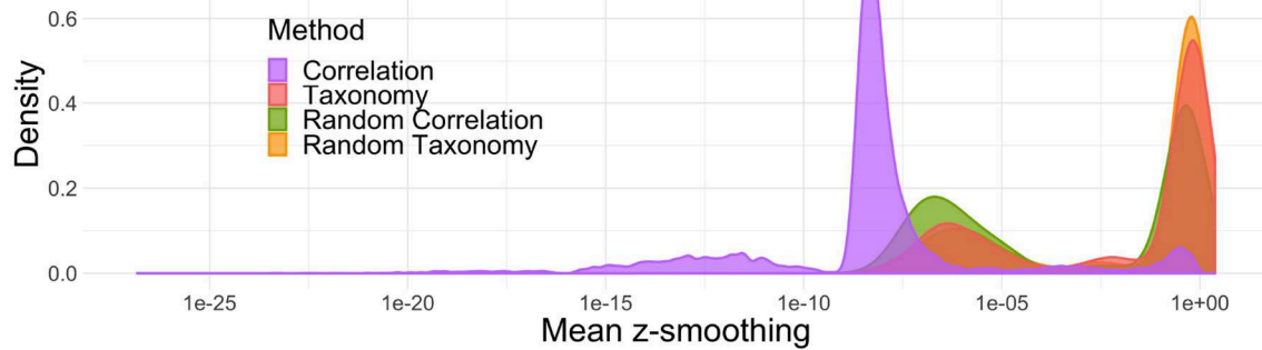
FIGURE 4 | Average absolute difference between z-scores before and after smoothing. In most simulations, smoothing only marginally changes the results.
