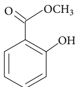
Methyl salicylate
