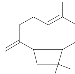
(E) - \beta -Caryophyllene
