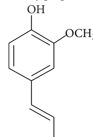
Eugenol
