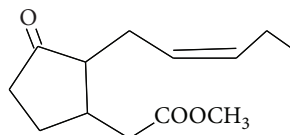
Methyl jasmonate “Green leaf volatiles”
