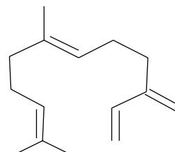
(E) - \beta -Farnesene
