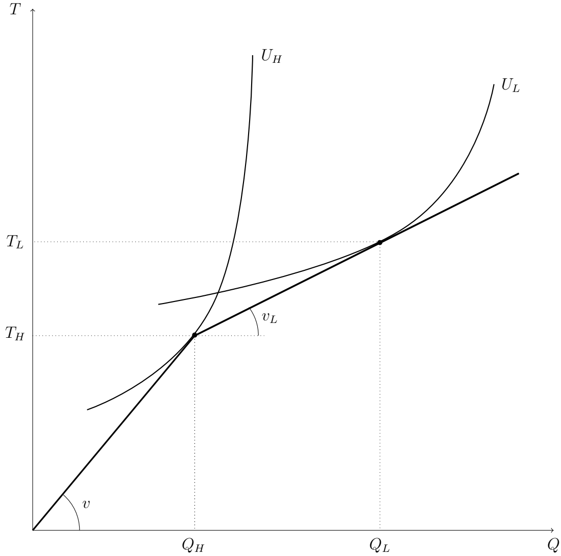
Figure 1 This figure depicts a candidate Jaynes–Hellwig–Glosten equilibrium with Q_L > Q_H > 0 .
