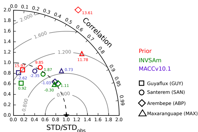
Figure 5. Taylor diagram of the statistics of misfits between observations and simulated CO 2 mole fractions between 12:00 and 15:00 LT at Guyaflex (square), Santarém (circle), Arembepe (diamond) and Maxaranguape (triangle), when wind speed > 2 m s -1 , using prior fluxes (red), INVSAm (green) and MACCv10.1 (purple). Radial distance from the origin: ratio of SD of simulated mole fractions and SD of the observations. Angle measured from the y axis: coefficient of correlation. Numbers next to the symbols: bias (in ppm). Grey circles: SD of the misfits (in ppm).
