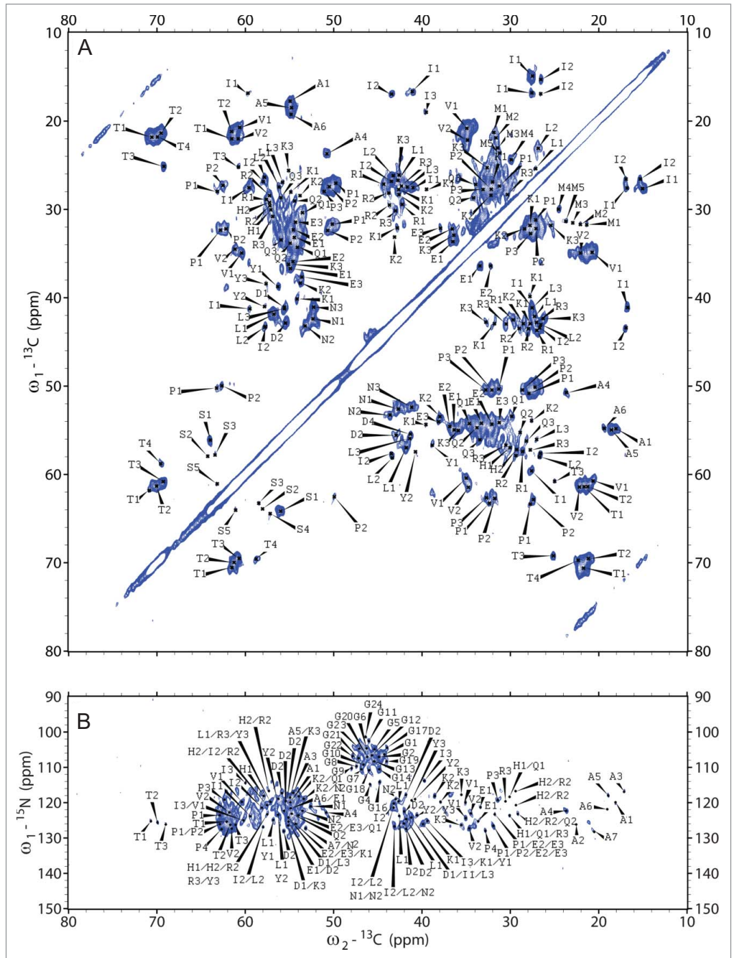
Figure 5. 2D-( 13 C- 13 C)- and ( 15 N- 13 C)-solid-state NMR correlation spectra. For identification of spin systems, homo- and heteronuclear correlation spectra were analyzed jointly. The aliphatic regions of (A) ( 13 C- 13 C)- and (B) ( 15 N- 13 C)-correlation spectra after spontaneous fibrillation of ovrecPrP(25-233) are depicted, acquired with (A) PDSM-mixing for 20 ms at 11 kHz MAS and (B) DREAM-mixing at 23 kHz MAS, to obtain intraresidue correlations. All cross peaks are labeled according to Tables S1, S2, and S3 . Note that in (B) several tentative assignments are present more than one time, reflecting the ambiguity as summarized in Table S3 .
