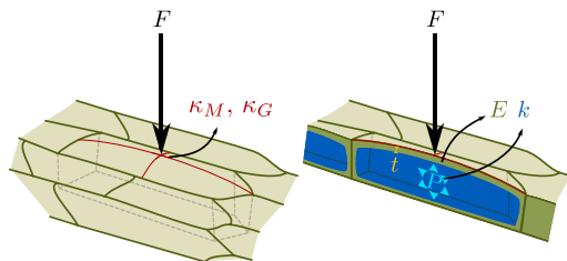
FIGURE 2 Schematics of the methodology to infer pressure: The topographic (height) image yields the local mean, \kappa_M , and Gaussian, \kappa_G , curvatures at the indentation point; the cell wall modulus, E , and the cell stiffness, k , are deduced from force-depth curves. Together with an independent measurement of wall thickness, t , these data enable the estimation of cell hydrostatic pressure, P . To see this figure in color, go online.
