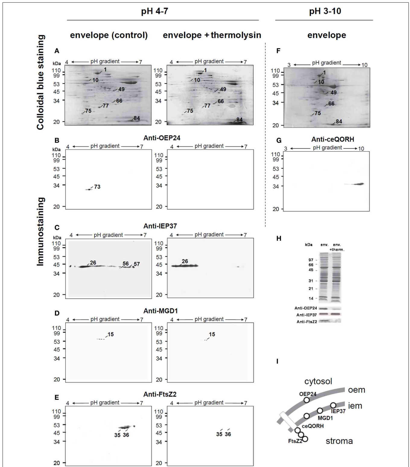
FIGURE 4 | Two-dimensional analysis of envelope proteins prepared from thermolysin treated intact spinach chloroplast. (A–D) Isolated intact spinach chloroplasts were incubated in the absence (control) or presence (+ thermolysin) of the non-permeable protease thermolysin. After chloroplast disruption, envelope sub-fractions were recovered. Envelope proteins
