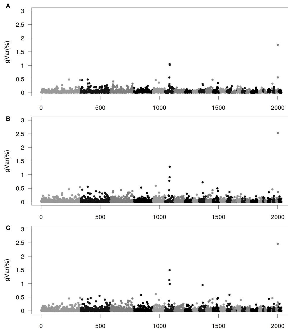
FIGURE 1 | Proportion of genetic variance of 20-SNP region under the Senarios 1 (ssGWAS1) of extended single-step genomic BLUP (ssGBLUP). (A) The first iteration (ssGWAS1/1). (B) The third iteration
