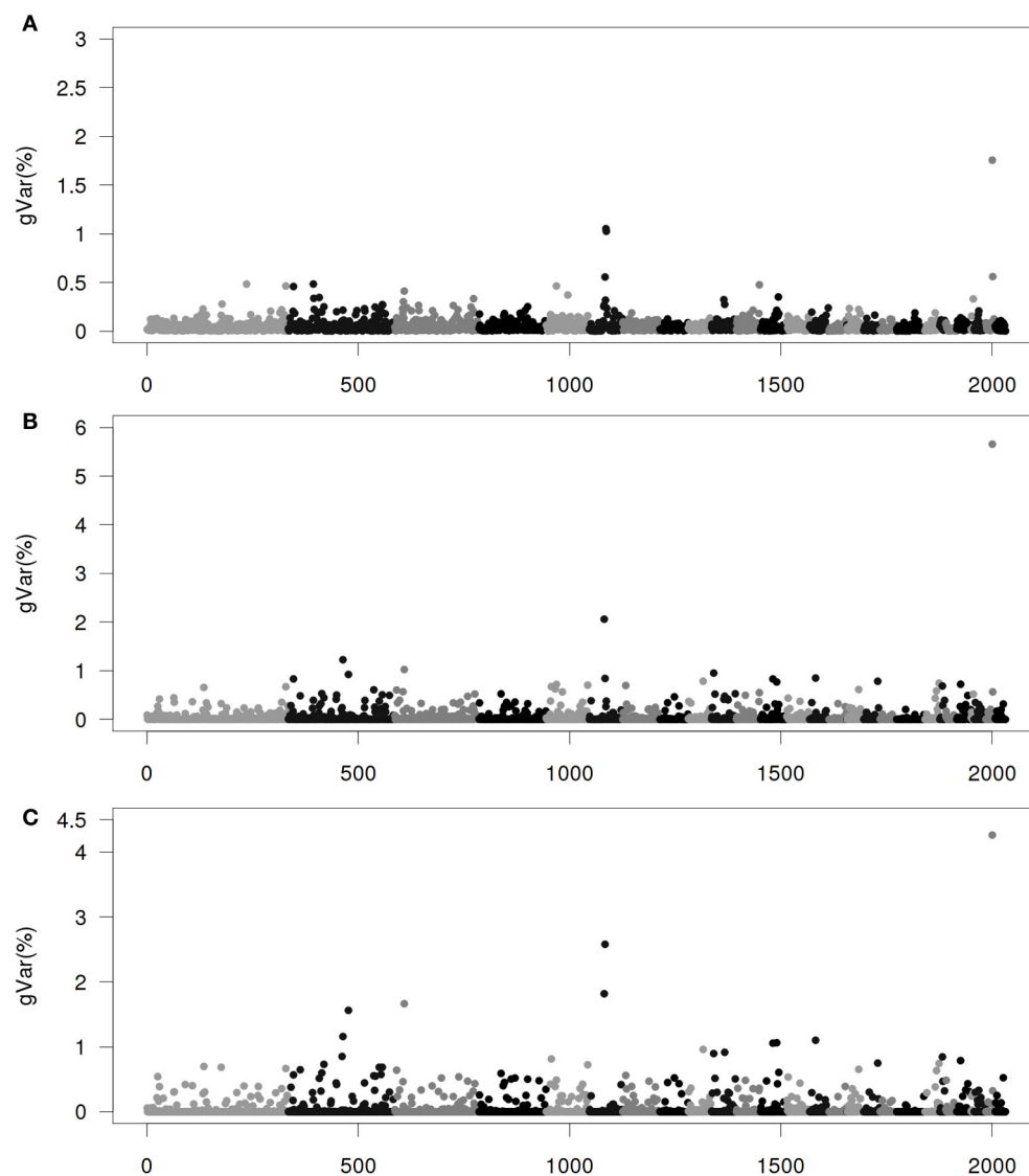
FIGURE 2 | Proportion of genetic variance of 20-SNP region under the Senarios 2 (ssGWAS2) of extended single-step genomic BLUP (ssGBLUP). (A) The first iteration (ssGWAS2/1). (B) The third iteration
