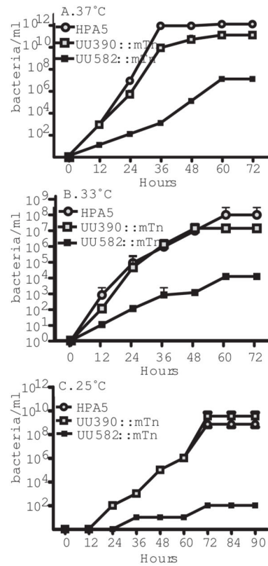
Figure 5. Growth kinetics for U. parvum parent strain (HPA5) compared to membrane protein disruption (UU390::mTn) or DEADbox RNA-helicase gene disruption (UU582::mTn) when incubated at 37°C (A.), 33°C (B.), or 25°C (C.). Strains were titrated out in a 10-fold dilution series and growth measured at time points indicated by urease conversion of urea to ammonium ions. Ureaplasma growth is shown as colour (pH indicator) changing units per ml. Mean and standard deviation of dilutions performed in triplicate. Results were consistent through three repeated experiments.
