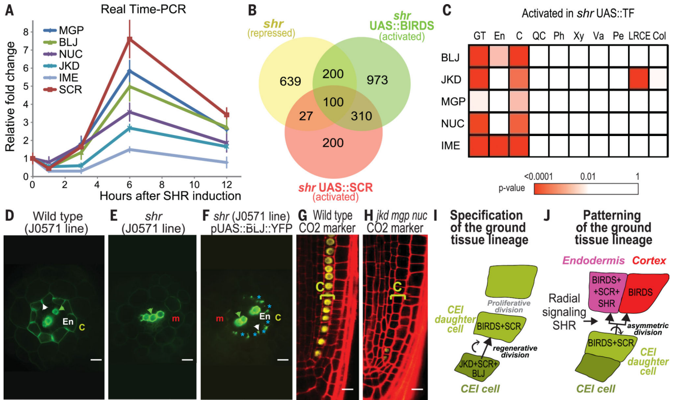
Fig. 4. BIRDs are activated by SHR and specify endodermis and cortex (A) BIRD expression in ground tissue cells at different times after SHR induction. (B) Venn diagrams comparing genes activated by BIRDs and SHR. (C) Heatmap of BIRD contribution to tissue-enriched expression. Ph: phloem; Xy: xylem; Va: vasculature; Col: columella. (D to F) Optical root sections at 10 dpi. White arrows: Casparian strip; green arrows: lignin in xylem. (G to H) Cortex marker in 6 dpi roots. (I and J) Model of postembryonic formation and maintenance of ground tissue. Scale bars: 10 \mu m.
