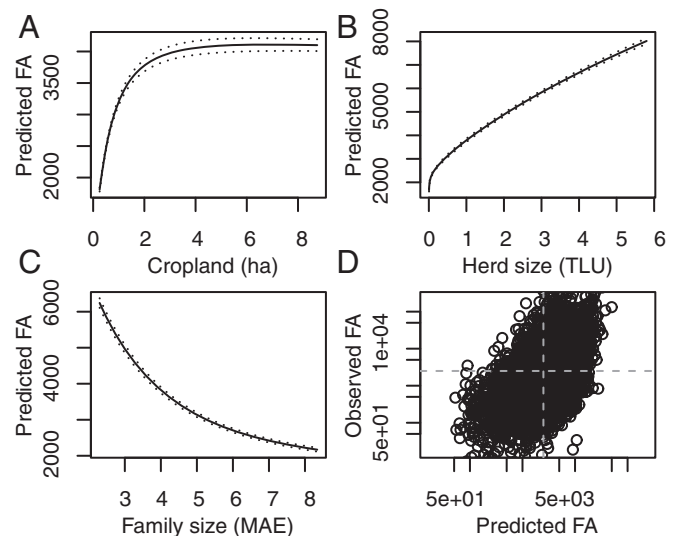
Fig. 4. (A–C) The response curves of the ANN model using cropland (A), TLUs (B), and family size (in MAE) (C) as inputs (on the x axes) and the predicted FA response (in kcal per capita per day) on the y axes. The curves were calculated from the controlled variation of one variable, whereas the other two were set to their median values: cropland, 1.33 ha; TLU, 0.75; and household size, 4.4 MAE. The bold line shows the average response curve, and the dashed line is the average \pm SD. (D) Model performance, with the observed FA (in kcal per capita per day; calculated using measured data) on the y axis and predicted FA (in kcal per capita per day) using the three earlier-mentioned variables as input of the ANN on the x axis. Both axes are in log scale. The dashed gray lines are the daily requirement thresholds of 2,500 kcal per capita per day (35).
