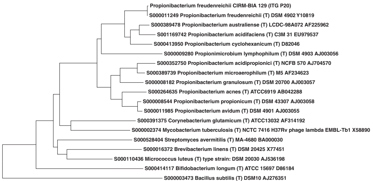
Fig. 2 The evolutionary history of the strain was inferred using the Neighbor-Joining method [12]. The optimal tree with a sum of branch lengths = 0.80 is shown. The tree is drawn to scale, with branch lengths in the same units as those of the evolutionary distances used to infer the phylogenetic tree. The evolutionary distances were computed using the Maximum Composite Likelihood method [13] and are in the units of the number of base substitutions per site. The analysis involved 18 nucleotide sequences. All positions containing gaps and missing data were eliminated. There were a total of 1376 positions in the final dataset. Evolutionary analyses were performed under MEGA5 [14]
