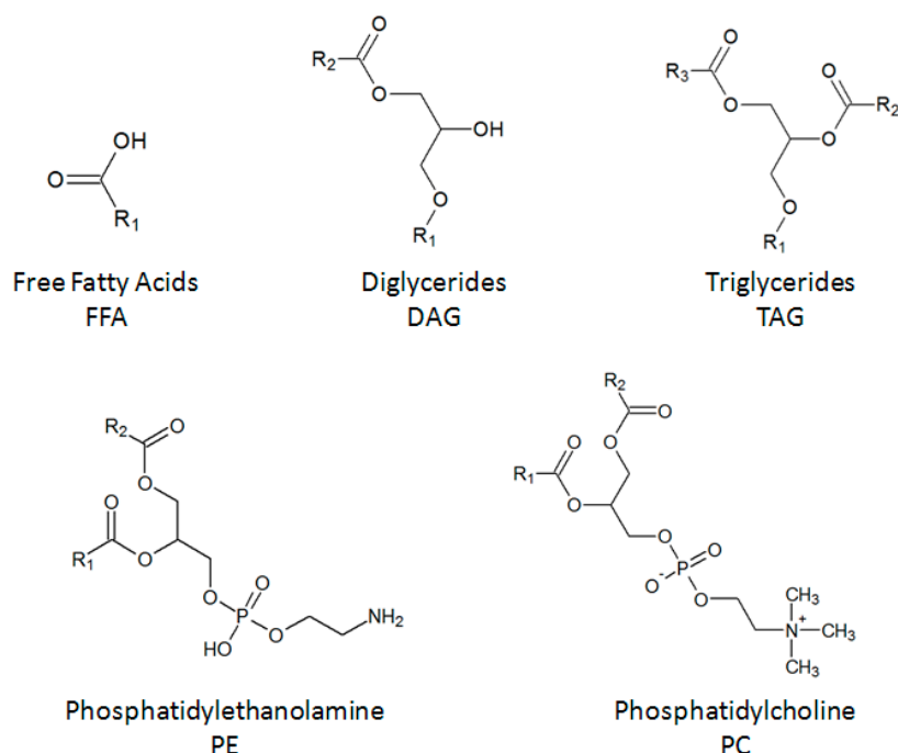
Figure 5. Structure of major lipids (FFA, DAG, TAG, PE, PC) found in yeast ( Yarrowia lipolytica ).
