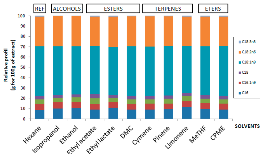
Figure 3. Comparison of the distribution of fatty acids by GC-FID to determine if there exists a selectivity during extraction.
