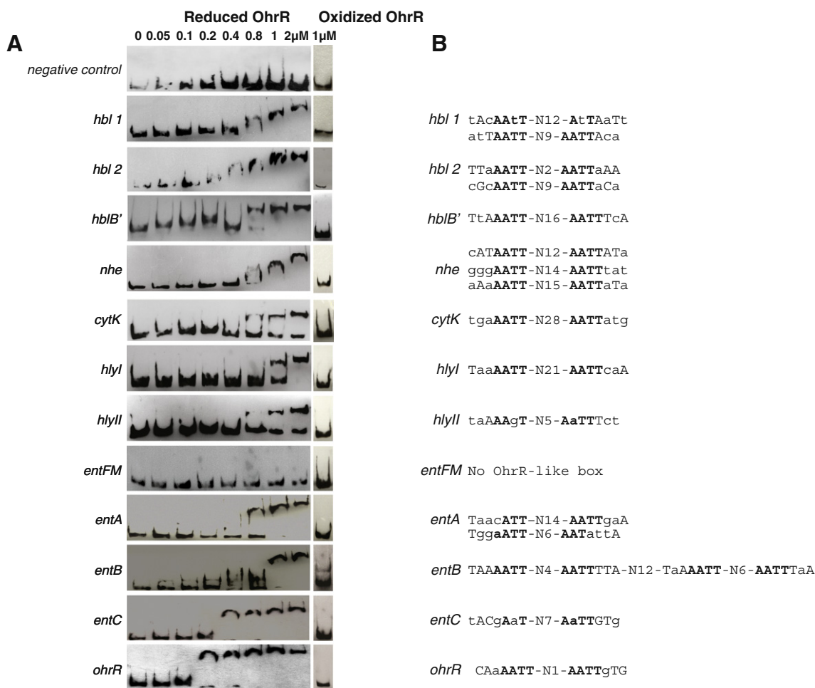
Fig. 4 – Binding of reduced and CHP-oxidized OhrR to toxin promoter regions determined by EMSA. Panel A. Biotin-labeled PCR products (2 nM) corresponding to hbl1 , hbl2 , hblB , nhe , cytK , hlyI , hlyII , entFM , entA , entB , entC , ohrR and a negative control (a fragment of the ssuRNA BC0007 sequence) were bound with 0, 0.05, 0.1, 0.2, 0.4, 0.8, 1 and 2 μM reduced OhrR and 1 μM CHP-oxidized OhrR. Panel B. Putative AT-rich OhrR binding sites upstream of toxin coding sequences are shown. Inverted repeats are shown in capitals. The core tetranucleotide AATT sequence of the consensus binding site of OhrR from other bacteria is indicated in capitals.
