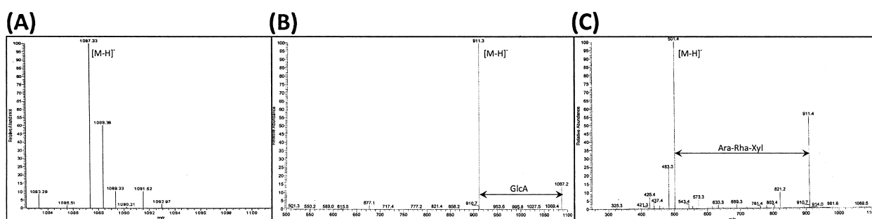
Figure 2 Negative-ion ESI-mass and tandem mass spectra of 3-O-[β-D-glucuronopyranosyl]-28-O-[β-xylopyranosyl(1 → 4)-α-L-rhamnopyranosyl(1 → 2)-α-L-arabinopyranoside] medicagenate (3-GlcA-28-AraRhxyl-medicagenate). (A) the ESI-mass spectrum of the isotope distribution of the (M-H) - ion at m/z 1087.33, of 3-GlcA-28-AraRhxyl-medicagenate, (B) MS/MS of 3-GlcA-28-AraRhxyl-medicagenate, precursor ion is m/z 1087.3, fragment ion at m/z 911.3 correlates to the loss of glucuronic acid (GlcA), (C) MS3 of 3-GlcA-28-AraRhxyl-medicagenate, precursor ion is m/z 911.3, fragment ion at m/z 501.4 correlates to the sequential loss of sugar substituents arabinose, rhamnose and xylose (Ara-Rha-Xyl) and thus the fragment ion at m/z 501.4 corresponds to M-H mass of medicagenic acid.
