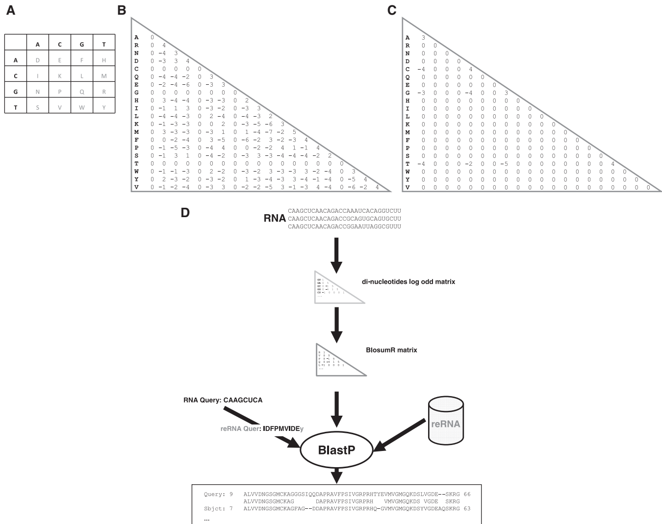
Figure 1. (A) Recoding scheme. The table shown represents the di-nucleotide to amino acid symbol recoding scheme. Rows correspond to the first letter of the di-nucleotide, while columns to the second. For example the di-nucleotide ‘AC’ is recoded to ‘E’. (B) BlosumR log-odd matrix. The matrix assigns a score for each possible substitution between di-nucleotides pairs. (C) BlosumN log-odd matrix. The matrix assigns a score for each possible substitution between nucleotides pairs. (D) BlastR pipeline. Rfam seed alignments are used to estimate a log-odd matrix (BlosumR). BlastP is then used along with BlosumR to search recoded RNA query sequences against a similarly recoded RNA database.
