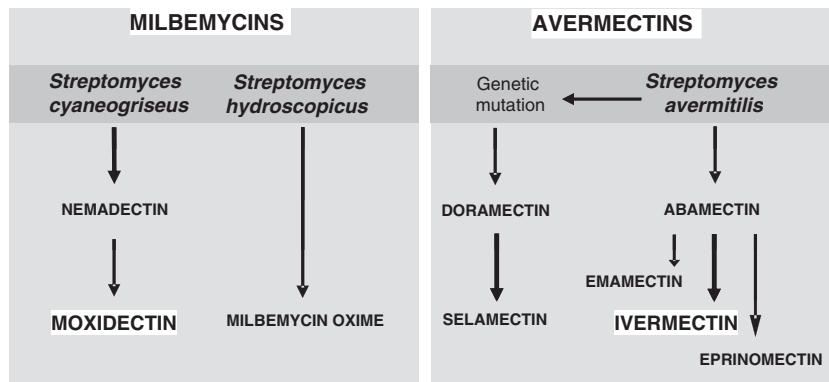
Fig. 1. Schematic filiations of macrocyclic lactones: from the soil bacteria to the therapeutic products.
