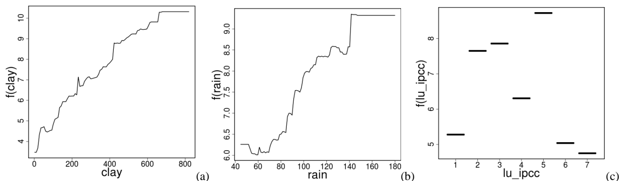
Fig. 6. Effect of the three most important variables in the Extra model (i.e. (a) clay , (b) rain and (c) lu_ipcc ). The lu_ipcc variable is coded using the adapted IPCC classification: croplands (1), permanent grasslands (2), woodlands (3) orchards, shrubby perennial crops (4), wetlands (5), others (6), vineyards (7).
