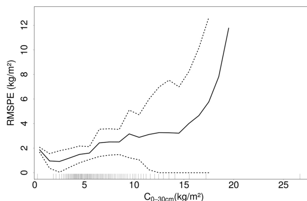
Fig. 4. Uncertainty of the Extra model, as a function of the organic carbon stock (30 cm). Uncertainty values (i.e. \langle \text{RMSPE}_{\text{ext}} \rangle , resulting from cross-validations trials) are calculated as a function of predicted SOC stocks, grouped within intervals of 1 \text{ kg m}^{-2} width, from 0 to 30 \text{ kg m}^{-2} . The solid line represents the mean of uncertainty within each interval of SOC stocks values, and the upper and lower dashed lines represent the bounds of the \text{CI}_{95\%} assuming a normal distribution within each interval. Tick marks at the lower border of the diagram give the 1% quantiles for the RMQS dataset.
