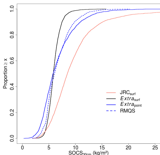
Fig. 3. Empirical cumulative distribution functions (ecdf) for the two spatial estimates presented in this paper (using the Extra model and the JRC estimate) as well as for the observed (curve RMQS) and predicted (curve Extra point ) SOC stocks at RMQS sites. Computing ecdf on spatial estimates is done as follows: first the statistical population is made of each spatial unit where the prediction model has been applied (the Extra model for instance). Second, a weight is computed for each unit as the ratio between its area and the sum of spatial units area (here, the area of France). Third, the ecdf is estimated on models predictions within the spatial units ( \text{kg m}^{-2} ) using weights previously calculated. Ecdfs of site observed or predicted values are calculated using equal weights between individuals.
