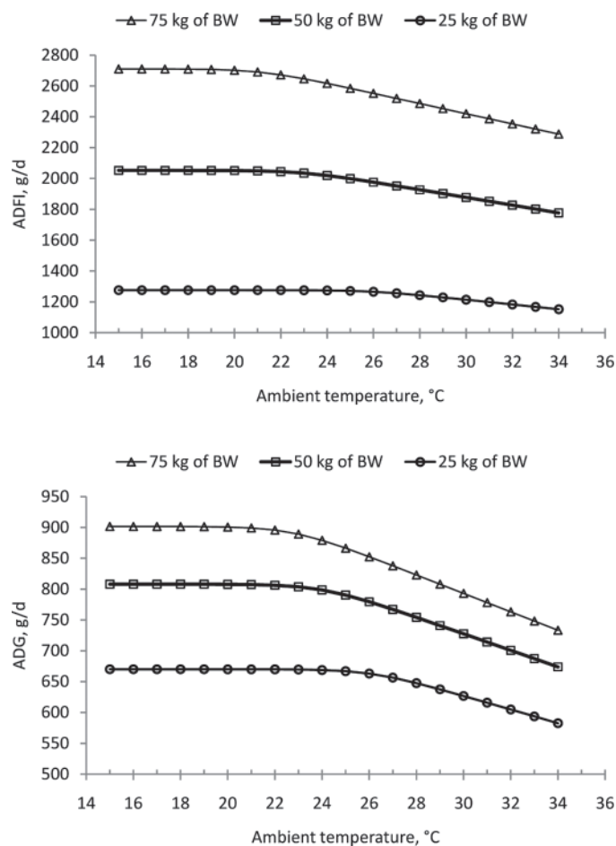
Figure 6. Effects of ambient temperature and pig BW on ADFI and ADG. The ADFI and ADG responses were calculated using the nonlinear models reported in Table 3.
