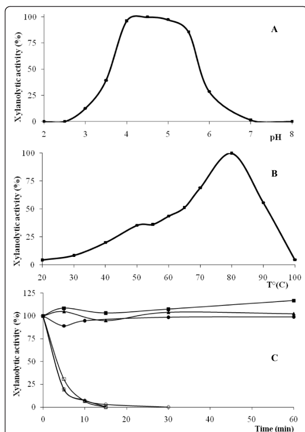
Figure 3 pH (A) and temperature (B) optima and thermostability (C) of XynD from P. funiculosum . (A) Effect of pH on the activity. Enzyme activity was assayed in a pH range of 2.0-8.0. (B) Effect of temperature on the activity. Enzyme activity was assayed at various temperatures of 20-100°C in 100 mM McIlvaine's buffer (pH 5.0). (C) Thermal stability of the enzyme. Thermal stability of the enzyme native (square) N-deglycosylated (triangle), N- and O-deglycosylated (circle) at 70°C (full symbol) and 80°C (empty symbol) were measured after incubation during several minutes at pH 5.0.
