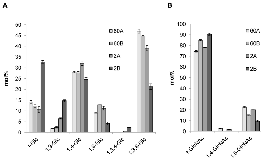
Figure 2. Linkage analysis of glucan-chitosaccharide fractions. The glycosidic linkages were identified by electron-impact mass spectrometry. Values are relative mole percentages (mol%) means \pm S.D. of 4 technical replicates. doi:10.1371/journal.pone.0075039.g002
