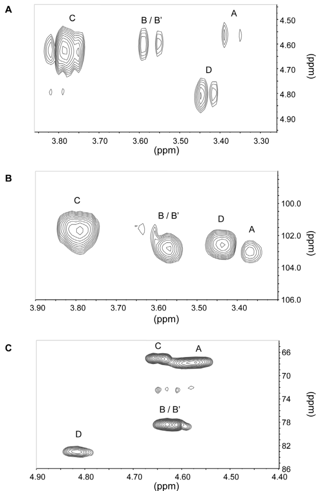
Figure 3. Two-dimensional liquid NMR spectra of glucan-chitosaccharide fraction 2B. A , Correlation spectroscopy (COSY) correlation (H-1/H-2) in the vicinity of anomeric protons; B , heteronuclear multiple bond coherence (HMBC) correlation in the vicinity of the C-1; C , heteronuclear multiple bond coherence (HMBC) correlation (C-3, C-4 and C-6/H-1) in the vicinity of the glycosidic linkages. Proton and carbon chemical shifts for units A, B/B', C and D are given in Table 4. doi:10.1371/journal.pone.0075039.g003
