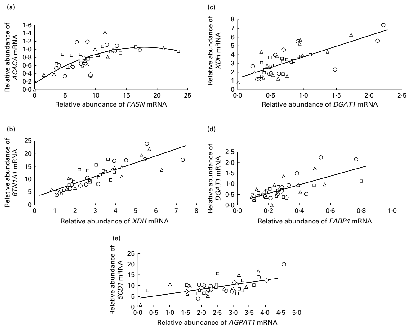
Fig. 1. Relationships between mRNA abundances of (a) acetyl-CoA carboxylase (ACACA) and fatty acid synthase (FASN): y = -0.0028x^2 + 0.0999x + 0.152 ; r = 0.72 , n = 42 , P = 0.01 ; (b) xanthine oxidoreductase (XDH) and butyrophilin (BTN1A1): y = 2.682x + 3.064 ; r = 0.84 , n = 42 , P = 0.01 ; (c) diacylglycerol acyltransferase 1 (DGAT1) and XDH: y = 2.405x + 1.358 ; r = 0.73 , n = 42 , P = 0.01 ; (d) DGAT1 and adipocyte fatty acid-binding protein (FABP4): y = 2.014x + 0.150 ; r = 0.71 , n = 42 , P = 0.01 and (e) 1-acyl- sn -glycerol-3-phosphate acyltransferase \alpha (AGPAT1) and stearoyl-CoA desaturase (SCD1): y = 2.167x + 3.893 ; r = 0.60 , n = 42 , P = 0.01 in the mammary gland of goats fed a diet with a high level of forage and supplemented with sunflower-seed oil (○) or a diet with a high level of concentrate with maize grain as source of starch and supplemented with sunflower-seed oil (□). The mRNA abundances are expressed in arbitrary units, determined as abundance relative to cyclophilin A mRNA and multiplied by 100.
