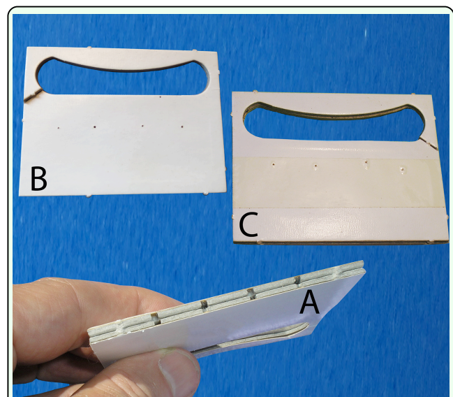
Figure 1. Dispensers used to release Trichogramma pretiosum in the field. A: usual dispenser with small holes on the edge; B: modified dispenser with very small holes on the side; C: modified dispenser improved with sticky tape at the level of the very small holes. High quality figures are available online.
