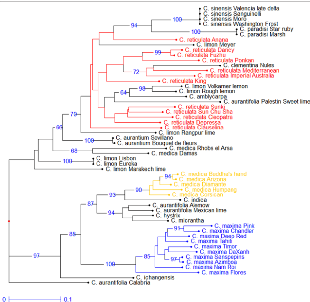
Figure 5 Neighbor Joining Analysis based on SNP loci with null alleles (WNA; 116 loci). Numbers near nodes are bootstrap values based on 1000 resamplings (only value > 60% are indicated).
