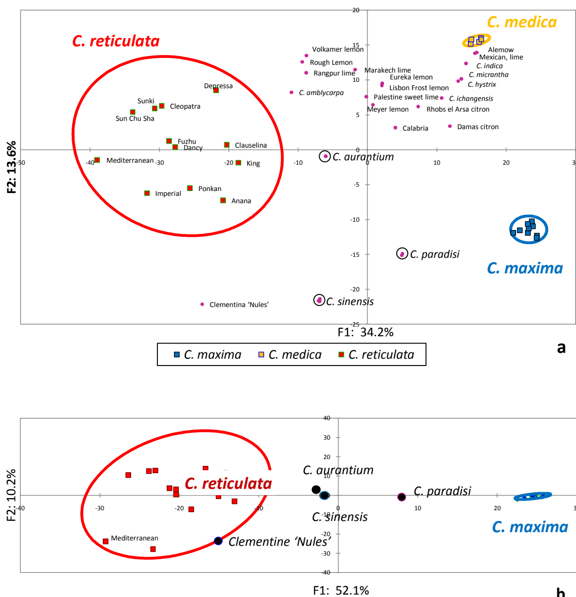
Figure 3 Principal component analysis from all loci without null alleles (506 loci). a) Axes 1/2 with all individual active. b) Positions of secondary species in the axis 1 of an ACP established from only C. reticulata and C. maxima as active accessions.
