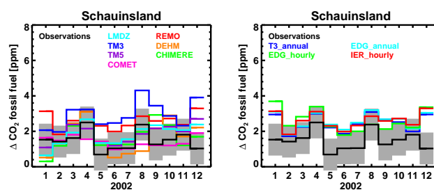
Fig. 6. Comparison of monthly-integrated fossil fuel CO 2 (relative to Jungfraujoch) at Schauinsland based on 14 CO 2 observations with simulations of all transport models using the “IER_hourly” emission inventory (left panel) and with simulations of the regional model REMO using the four different emission inventories (right panel). An uncertainty estimate of observed monthly mean fossil fuel CO 2 is included (grey shading).
